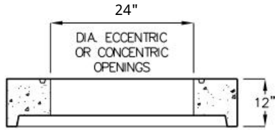
OPTIONAL FLAT TOP COVER
